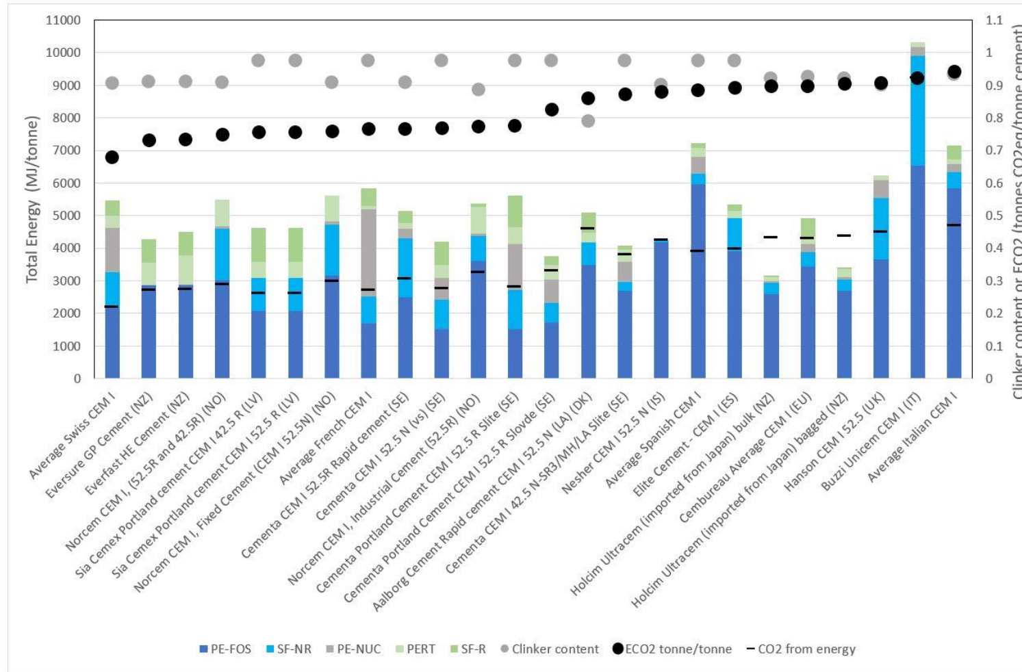
Figure 2 GWP, Energy Use and Clinker content for CEM I cements ( Anderson and Moncaster, 2020)
