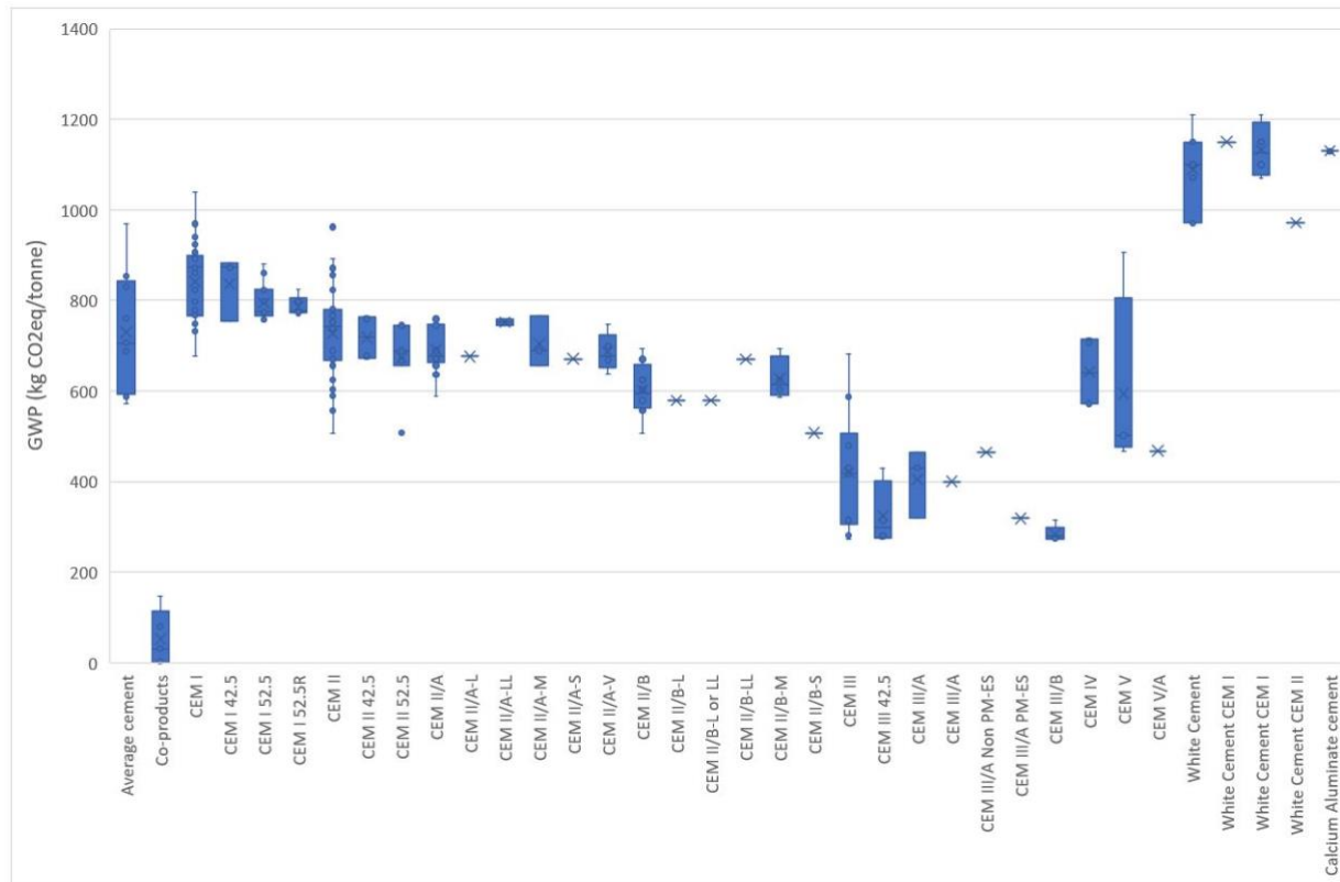
Figure 1 Variation in GWP (A1-A3) for different cements (Anderson and Moncaster, 2020)
