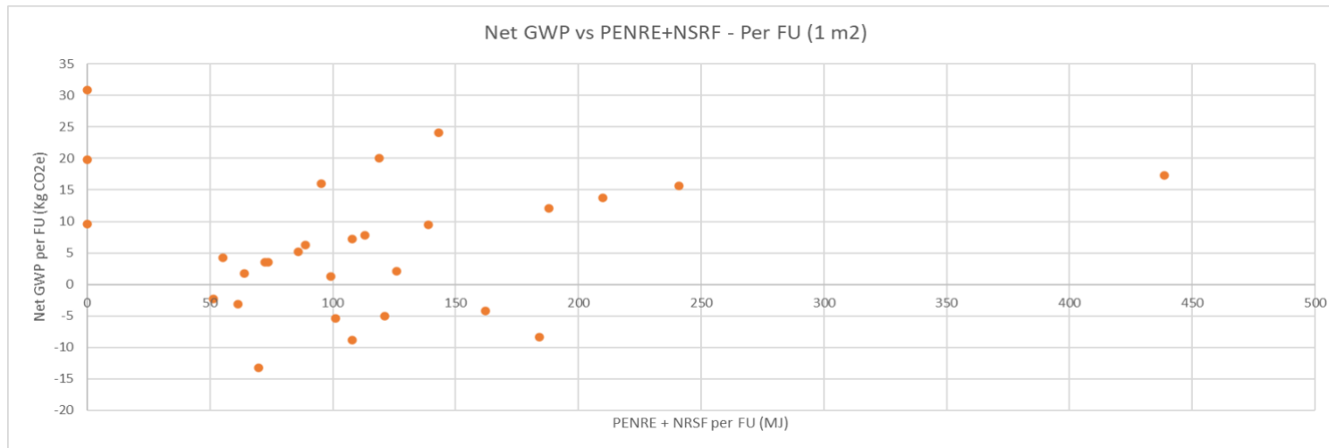
Figure 11 GWP v PENRT+NRSF per m2 for timber panel products
