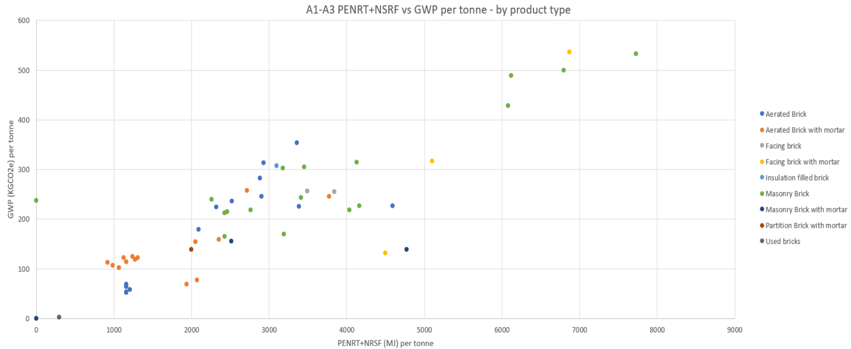
Figure 9 GWP v PENRT+NRSF per tonne for brick products
