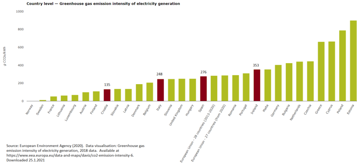
Figure 12 Greenhouse gas emission intensity of electricity generation by country
