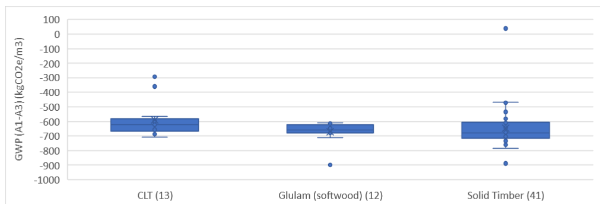
Figure 17 GWP (A1-A3) including sequestered carbon from structural timber EPD
