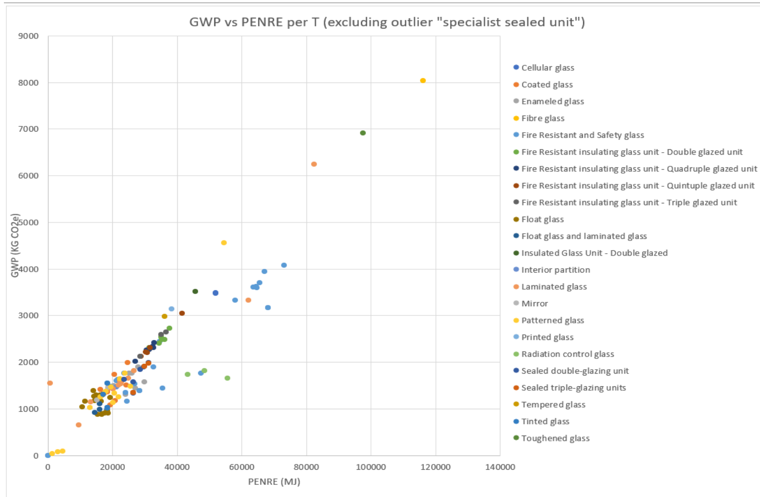
Figure 8 GWP (A1-A3) v. non-renewable primary energy v for glass products
