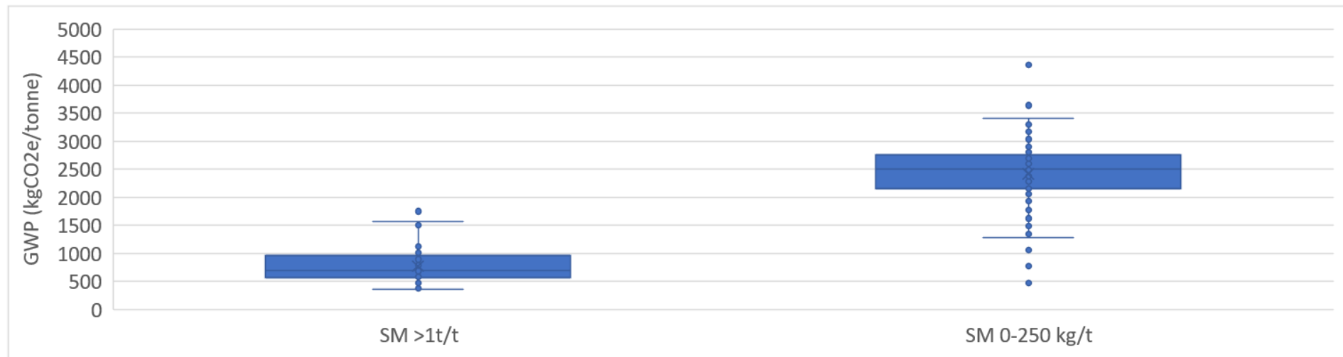
Figure 6 GWP (A1-A3) for steel EPD grouped by reported use of secondary material
