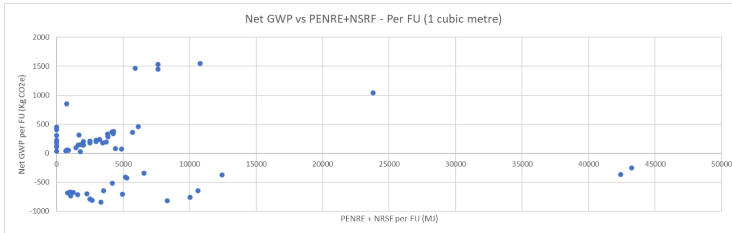
Figure 10 GWP v PENRT+NRSF per m3 for solid timber
