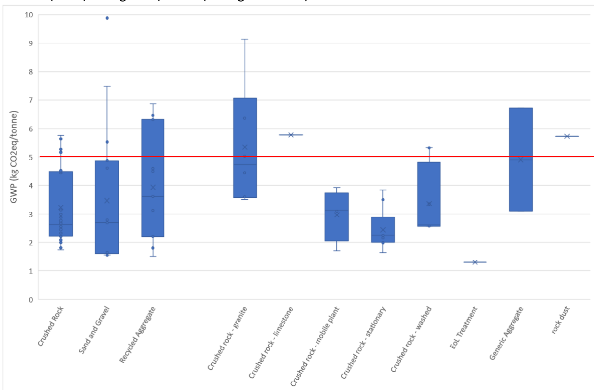
Figure 14 GWP for aggregate EPD from Anderson & Moncaster, 2020 showing the proposed value for Aggregate in Ireland
