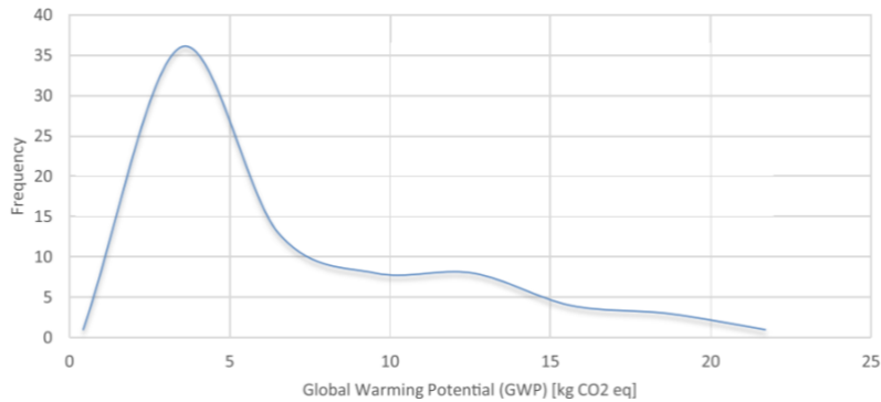
Figure 31 Distribution curve for GWP/unit of thermal performance (A1-A3) for 79 insulation products from Welling and Ryding, (2020)
