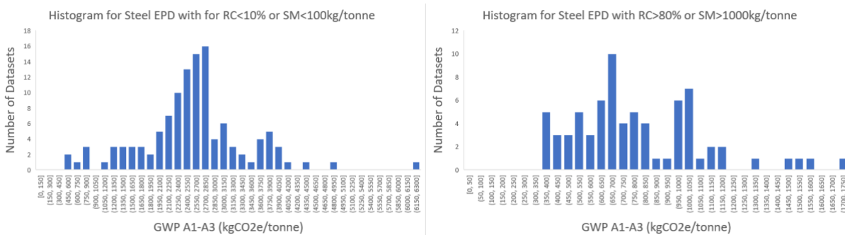
Figure 38 Histograms showing distribution of steel EPD with different recycled content or use of Secondary Material
