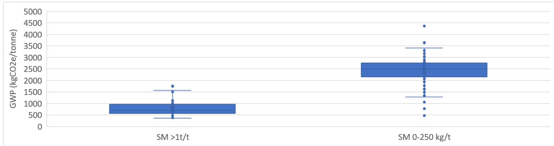
Figure 6 GWP (A1-A3) for steel EPD grouped by reported use of secondary material
